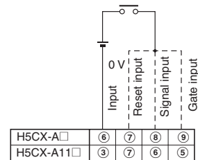
Operate with relay ON
